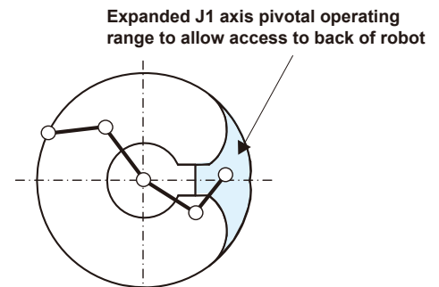
Rear access of RH-FQ/FD
